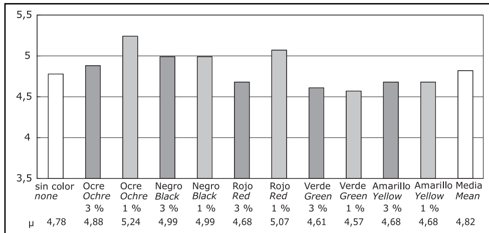
Figura 2. Resistividad relativa para muestras de YF amasadas con A/Y= 0,8. Figure 2. Relative resistivity for FP samples with a W/P ratio of 0.8.
