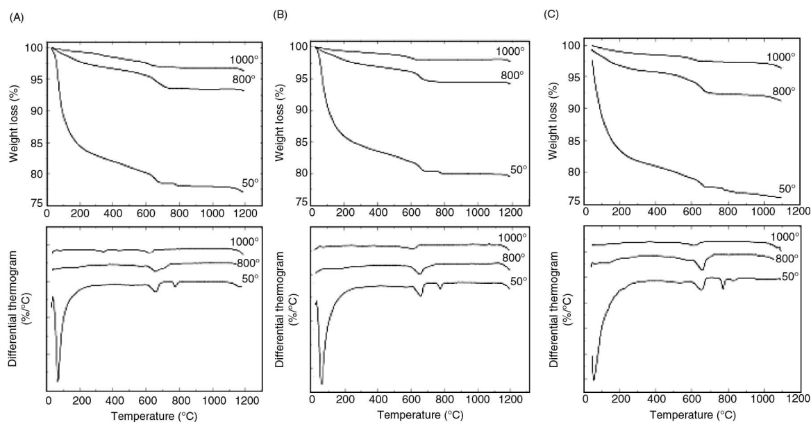
FIGURE 5. Thermograms (top) and differential thermograms (bottom) of alkali-activated slag pastes activated with (A) commercial sodium silicate, (B) silica fume-based activator and (C) rice husk ash-based activator, as a function of the temperature of exposure.
