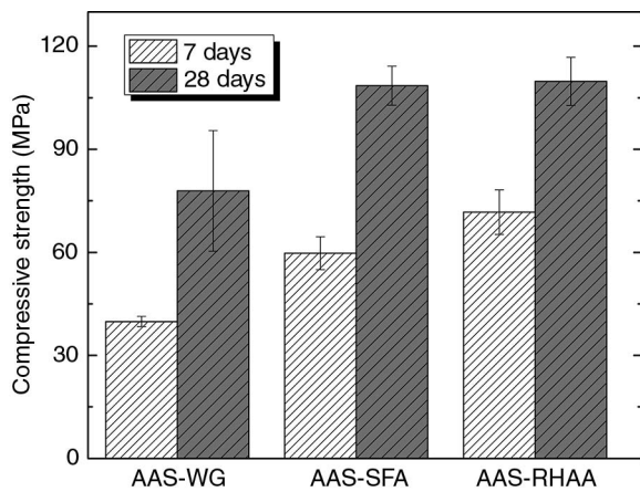
FIGURE 1. Compressive strength of slag pastes activated with different silicate solutions.
