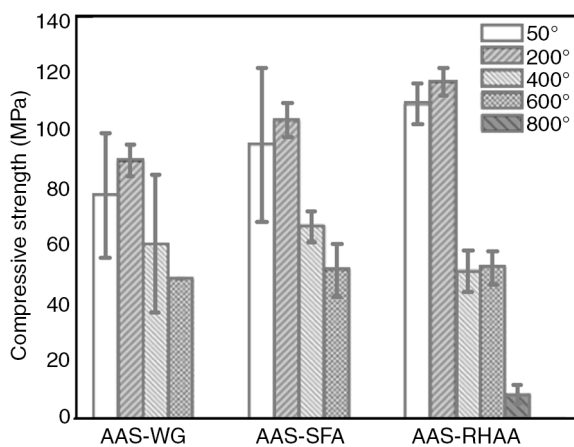
FIGURE 2. Compressive strength of activated slag exposed to high temperatures as a function of the silicate activator source.
