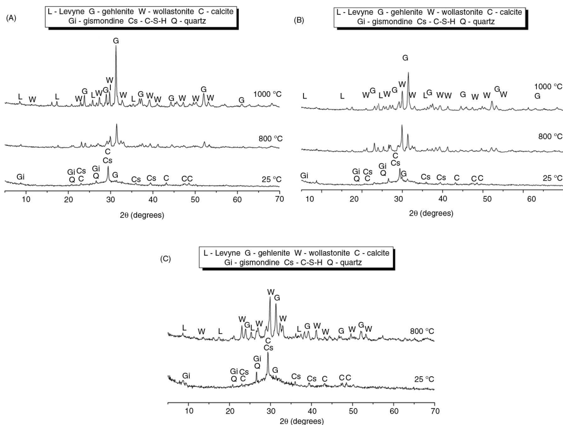
FIGURE 4. X-ray diffractograms of alkali-activated slag pastes activated with (A) commercial sodium silicate, (B) silica fume based activator and (C) rice husk ash based activator, as function of the temperature of exposure.
