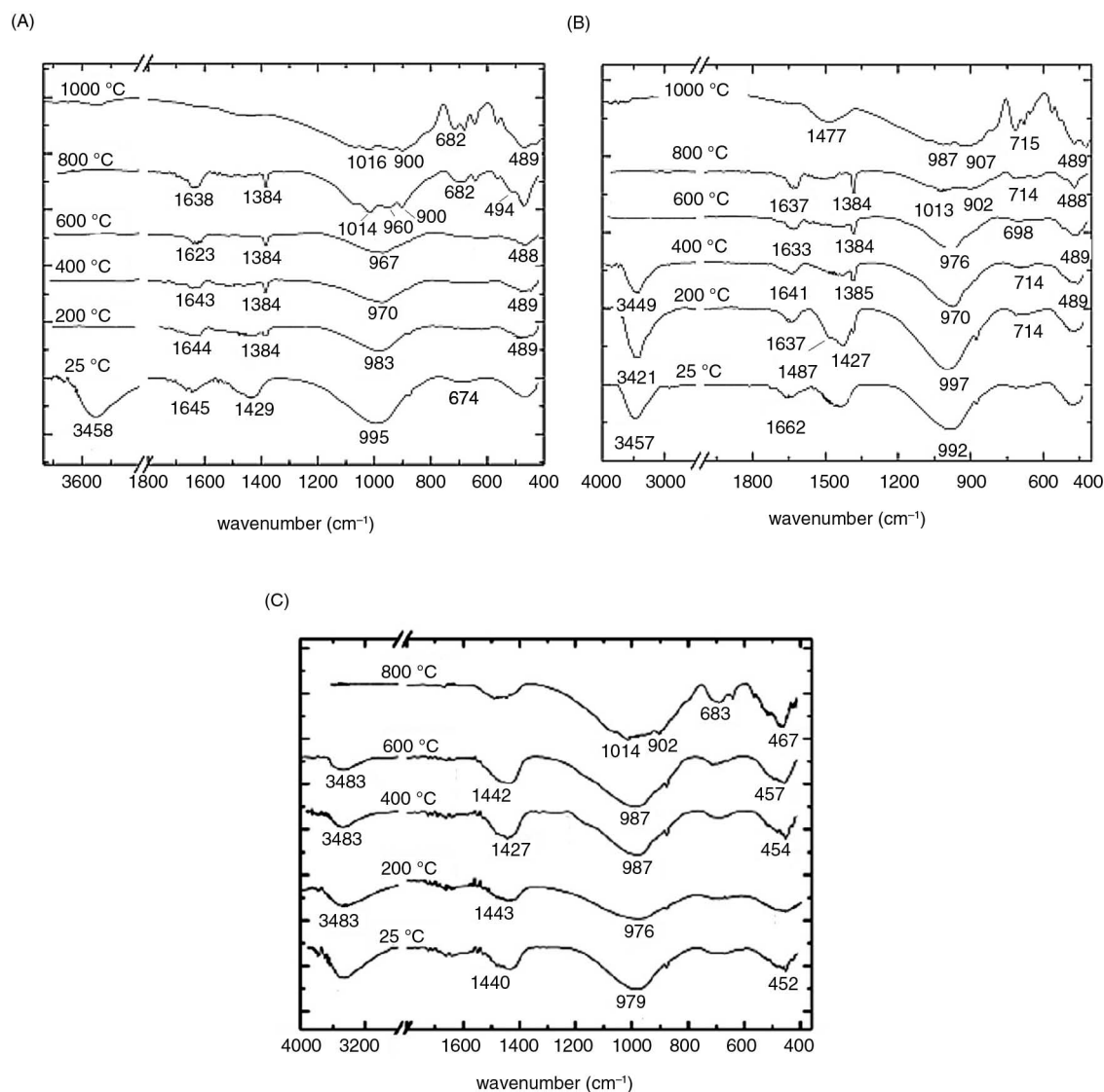
FIGURE 6. Fourier transform infrared spectra of alkali-activated slag pastes activated with (A) commercial sodium silicate, (B) silica fume based activator, and (C) rice husk ash based activator, as a function of the temperature of exposure.
