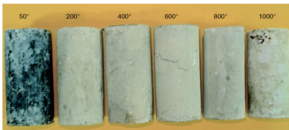
FIGURE 3. Photograph of RHA-activated slag specimens exposed to different temperatures. The green colour of the sample treated at 50 °C is intrinsic to the slag-rich binder, and converts to white upon heating due to oxidation processes. The cracks in samples heated above 600 °C are clearly visible.
